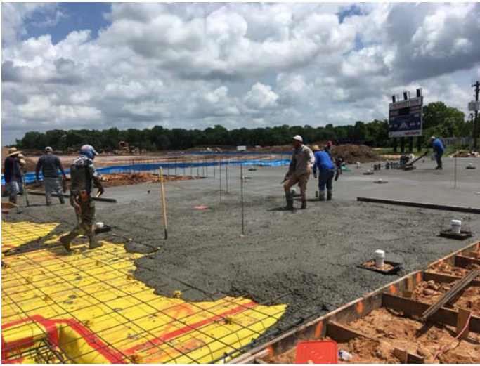
7. Concrete slab on grade at concessions
