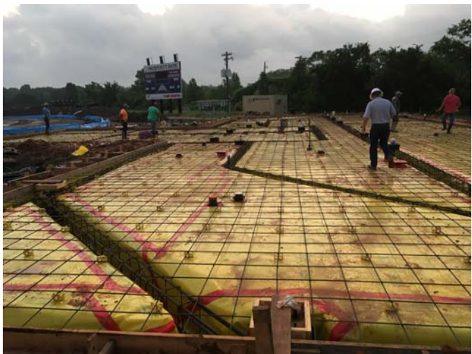
5. Slab on grade prep complete
